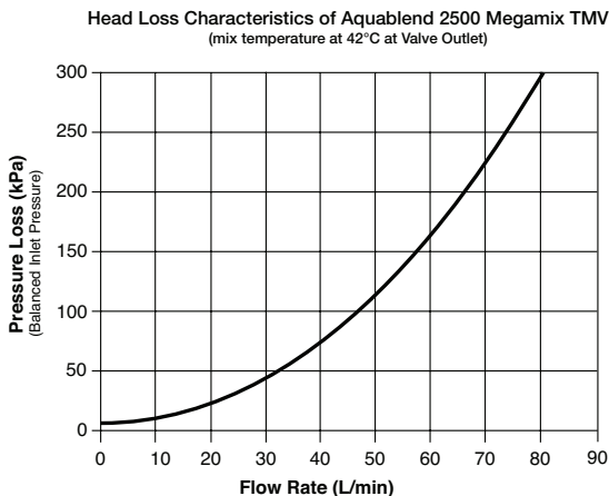
IMAGE 3 - Headloss Characteristics
