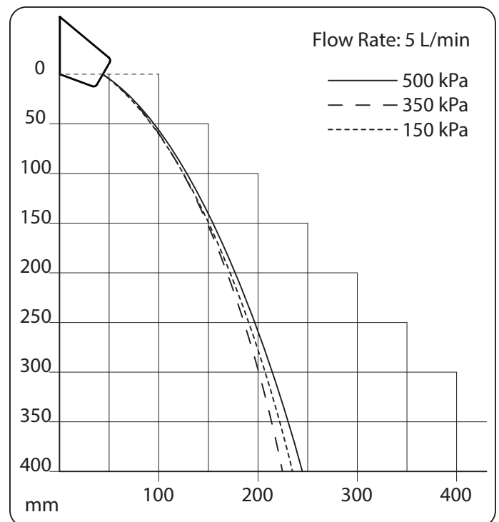
BASIN OUTLET FLOW PROJECTION
